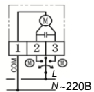
VGFA010FL VGFA015FL
