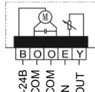
VGFA010R VGFA015R
