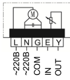
VGFA018RL VGFA030RL
