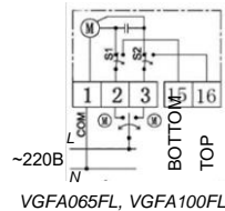
VGFA065FL, VGFA100FL
