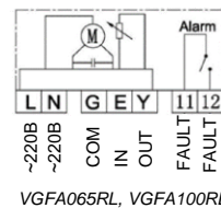
VGFA065RL, VGFA100RL
