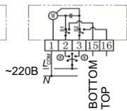
VGFA018FL VGFA030FL
